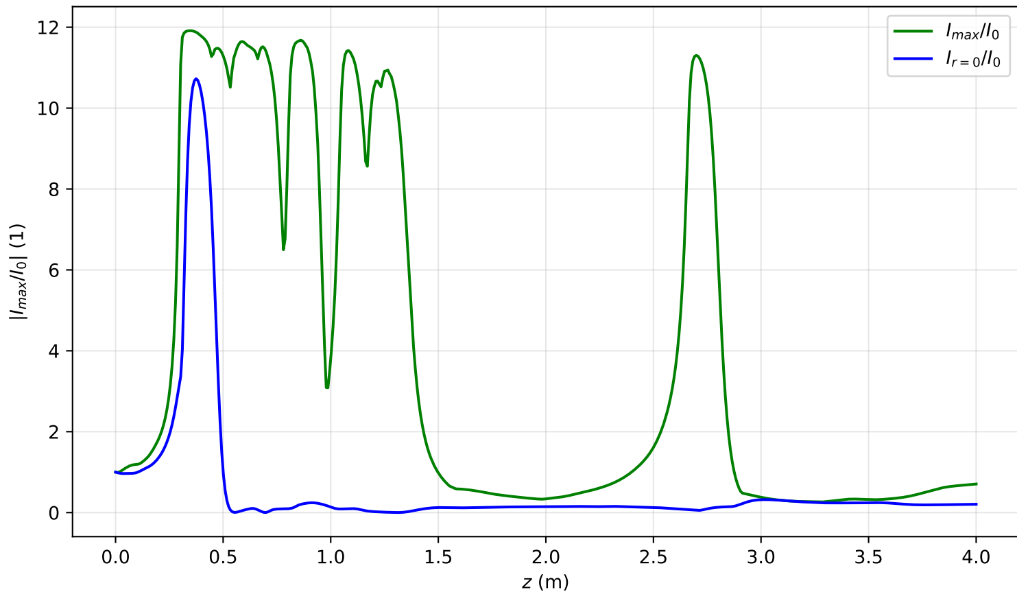
I_{max}(x = 0, y = 0, z)/I_0 , \text{Pin}=9.3\text{Pcr} , noisy input, artificial time
